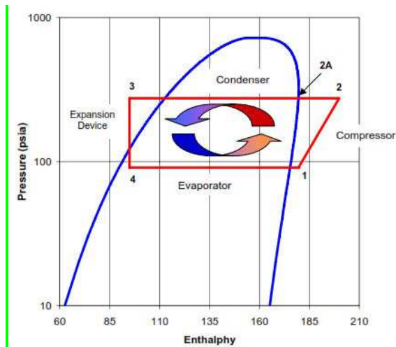
Figure 2: P-H diagram
