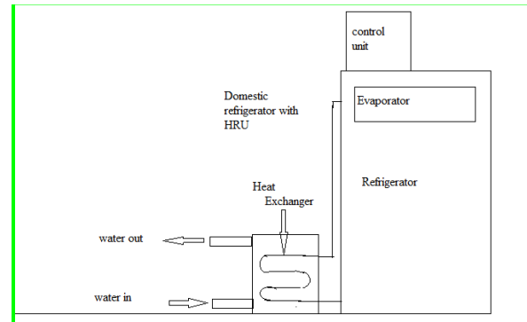
Fig 3:- system layout
