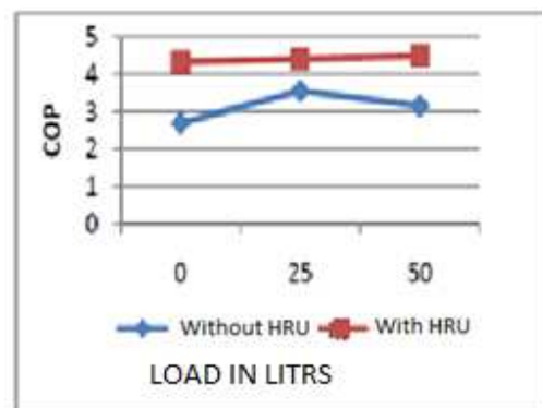
Fig.5 Theoretical COP Vs. Load
